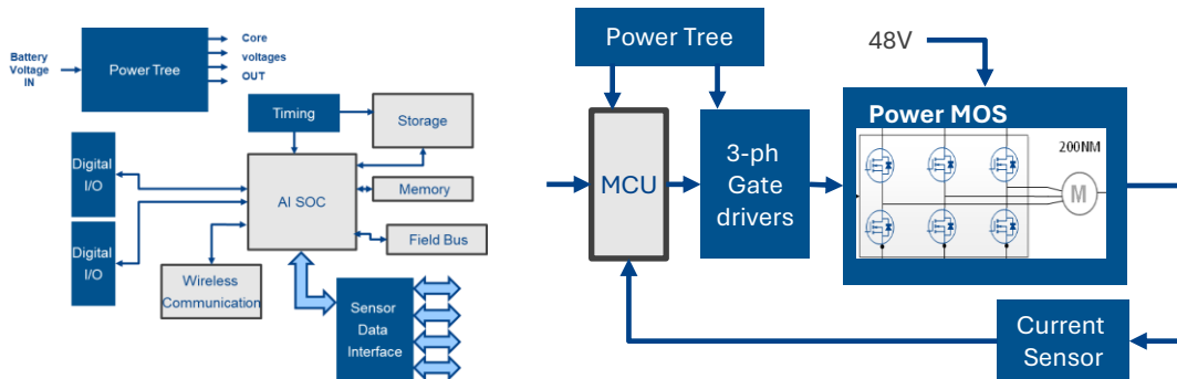
3 Phase Bionic Joint Motor
